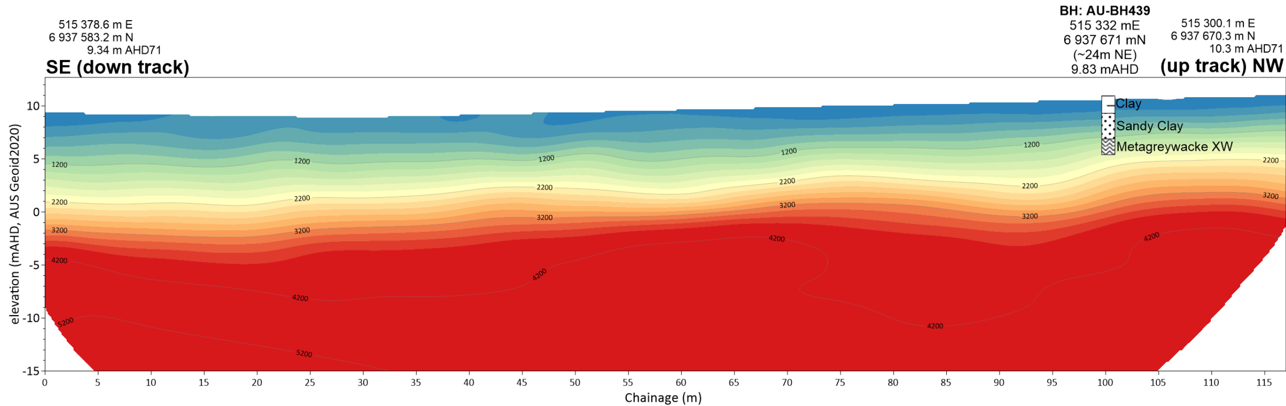
Seismic Line SR AU-GP 165-4
